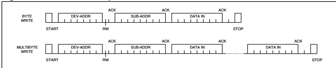
Figure 14. Write mode sequence
